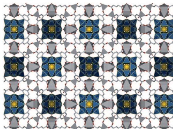
Figure 21. [Cu_2(btc)_{4/3}(H_2O)_2]_6[H_nXM_{12}O_{40}] , which contains Keggin ions as non-coordinating guests within a framework. W blue, X yellow, O red, C gray, Cu gray polyhedra.
